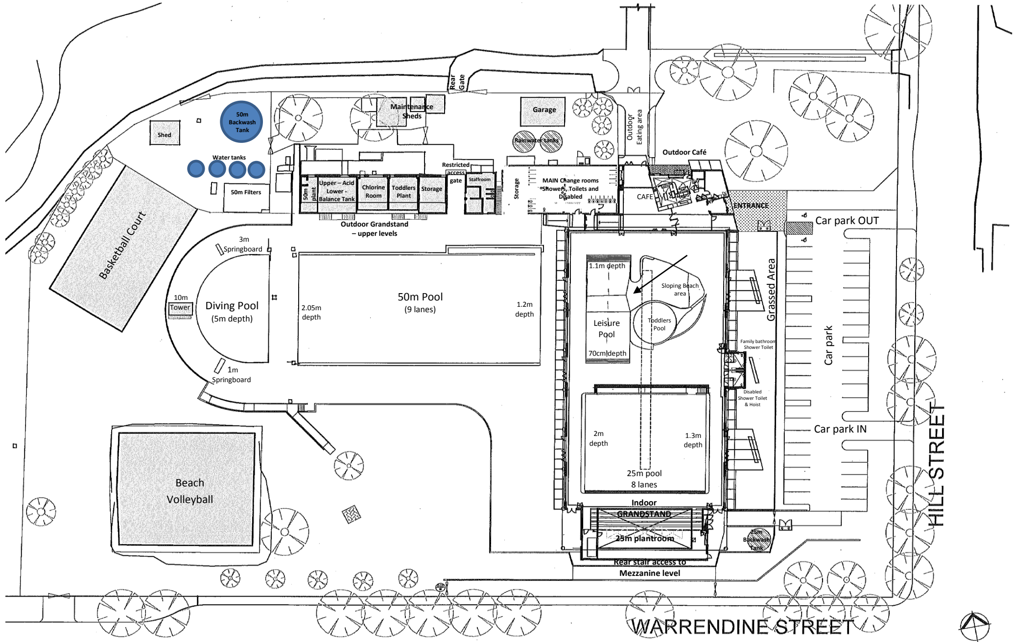
Orange Aquatic Centre – Facility Layout – V1 BS110517
